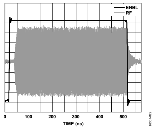
Figure 22. Enable/Disable Time Domain Response
