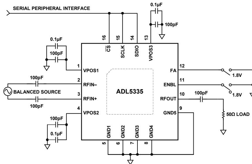
Figure 25. Basic Connections
