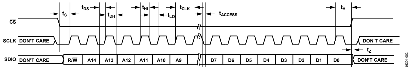
Figure 2. SPI Timing
