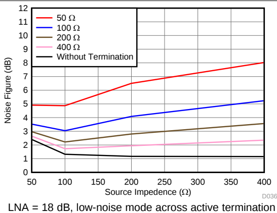
Figure 36. Noise Figure vs Source Impedance
