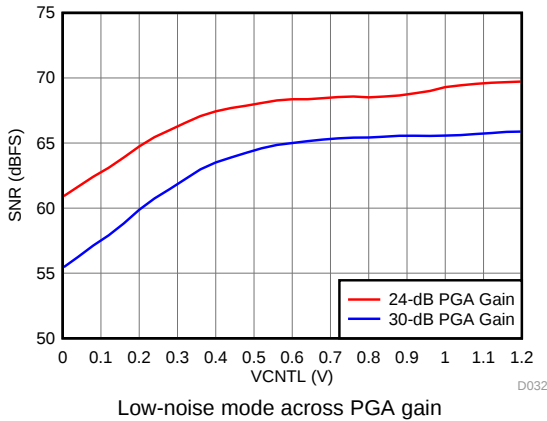
Figure 32. Signal-to-Noise Ratio vs VCNTL
