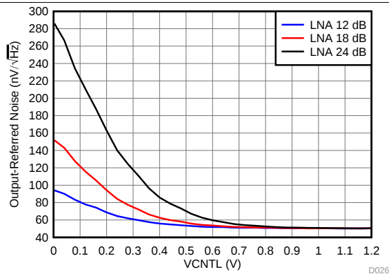
Figure 26. Output-Referred Noise vs VCNTL
