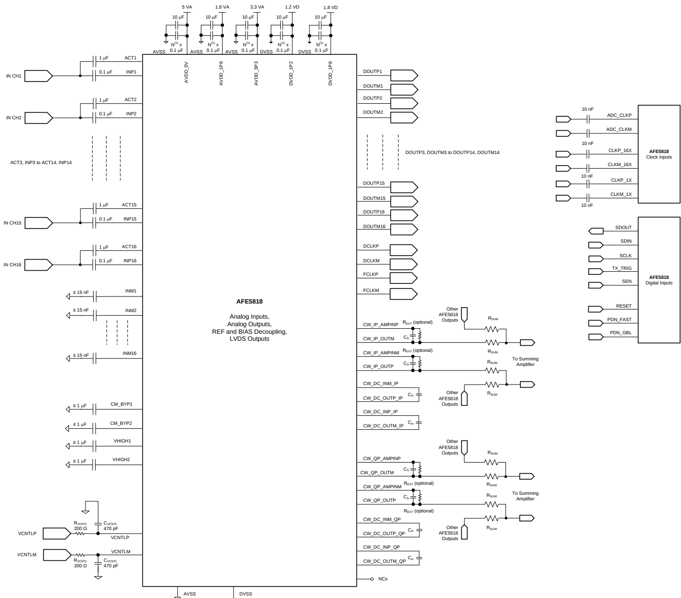
Figure 104. Application Circuit
