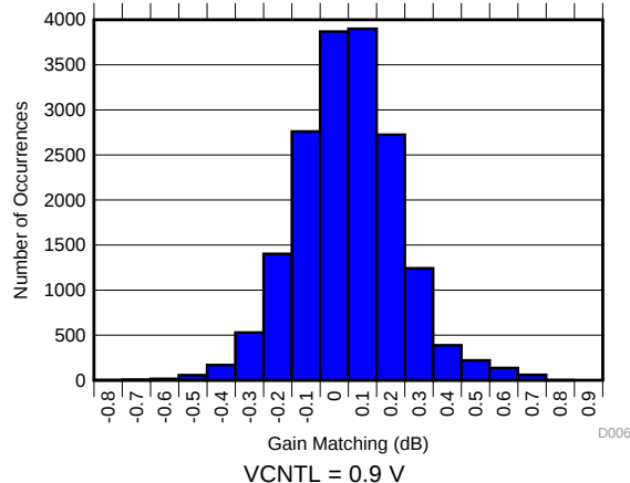
Figure 6. Gain Matching Histogram (17472 Channels)
