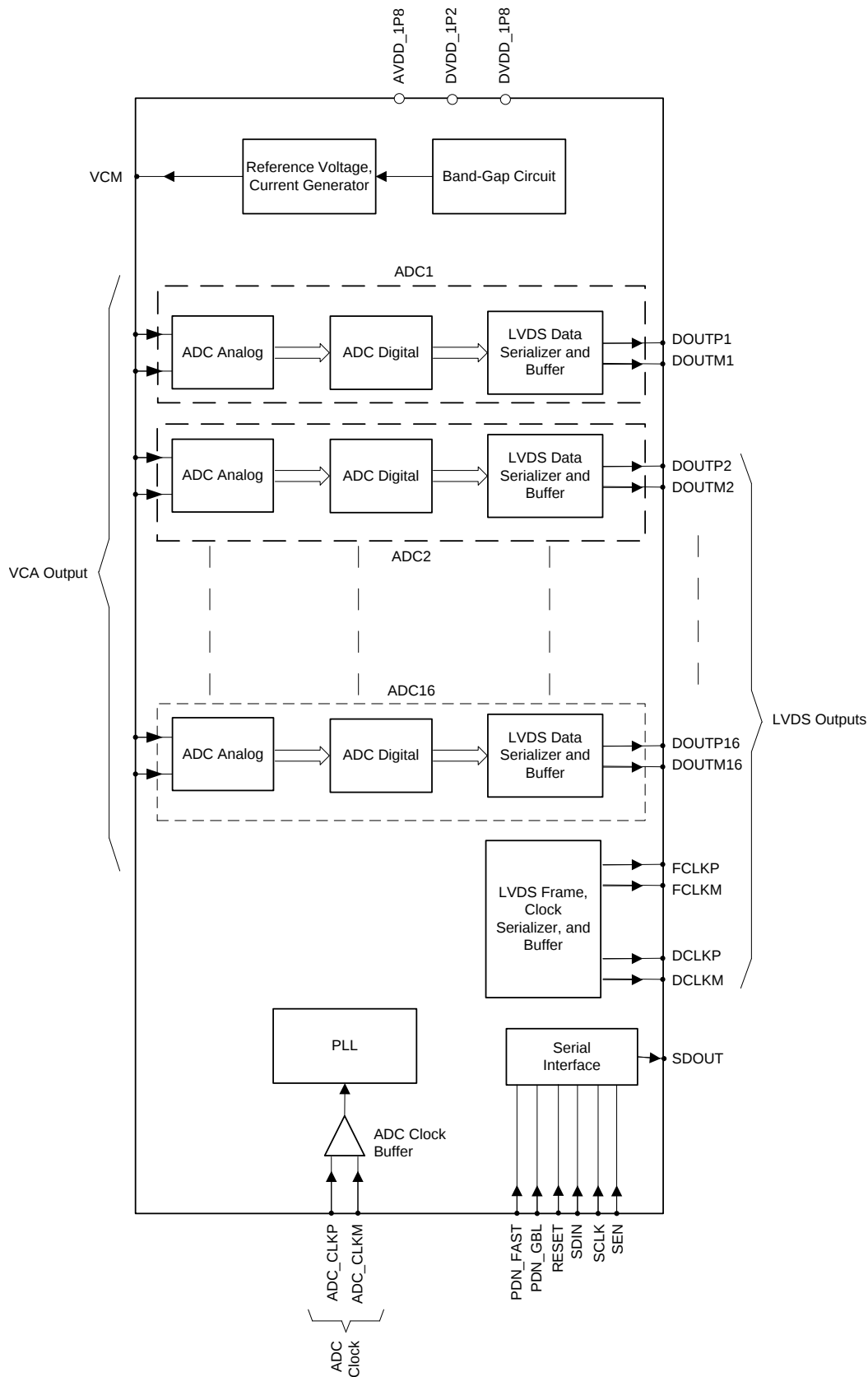
Figure 99. ADC Block Diagram
