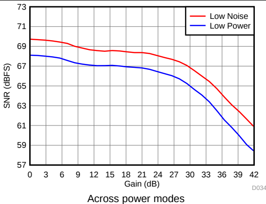
Figure 34. Signal-to-Noise Ratio vs Gain
