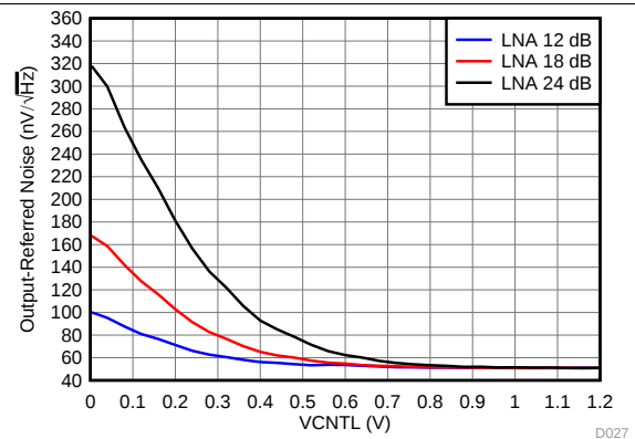
Figure 27. Output-Referred Noise vs VCNTL
