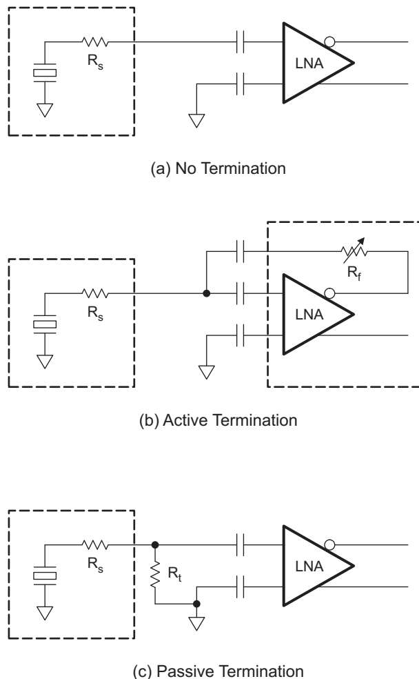
Figure 64. Termination Configurations
