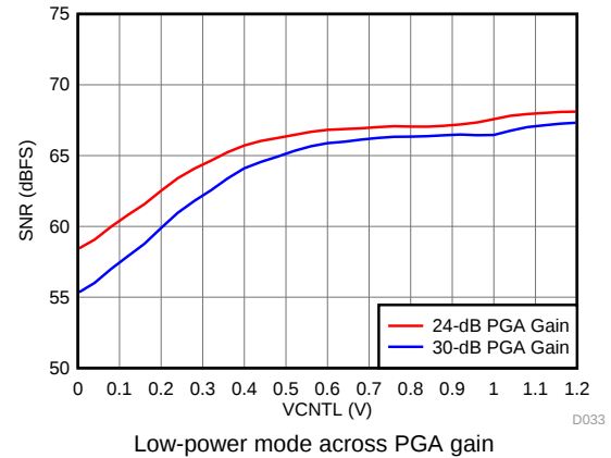
Figure 33. Signal-to-Noise Ratio vs VCNTL
