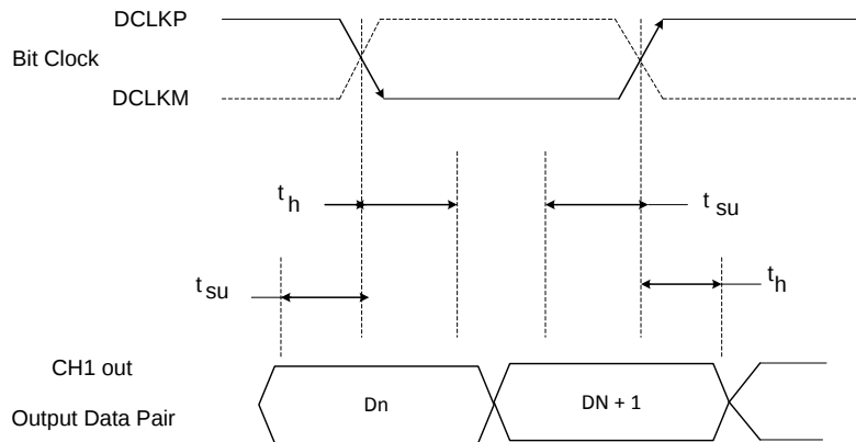
Figure 77. LVDS Timing Nomenclature
