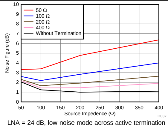
Figure 37. Noise Figure vs Source Impedance
