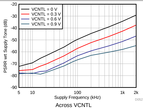
Figure 52. AVDD Power-Supply Rejection Ratio vs 100-mV PP Supply Noise Frequencies
