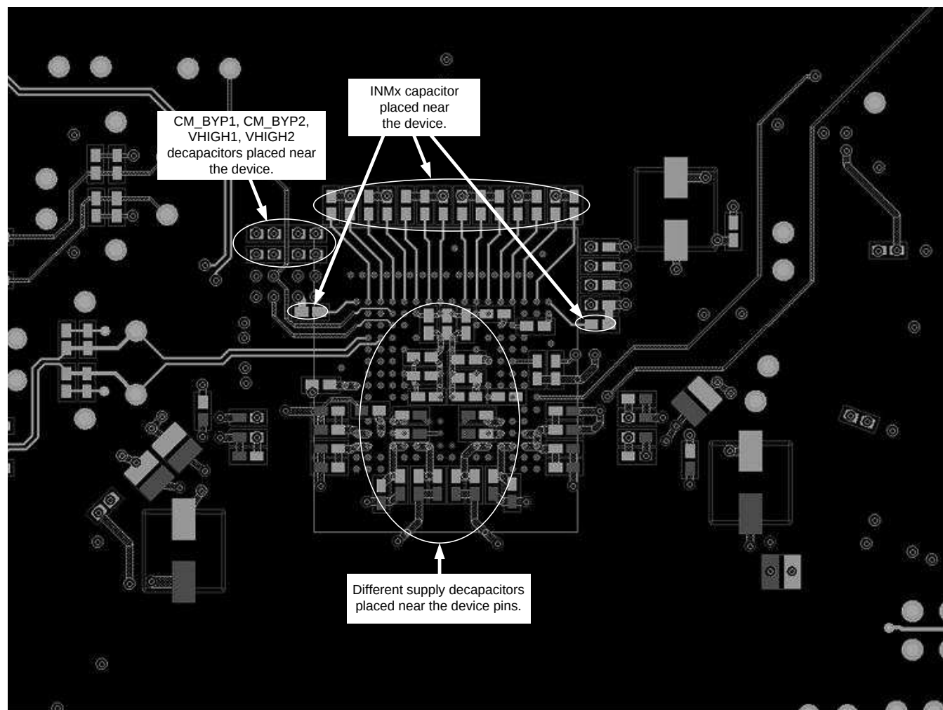
Figure 109. Bottom Layer
