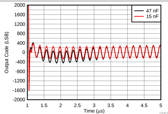
Figure 59. Device Pulse Inversion Output vs Time (Zoomed)
