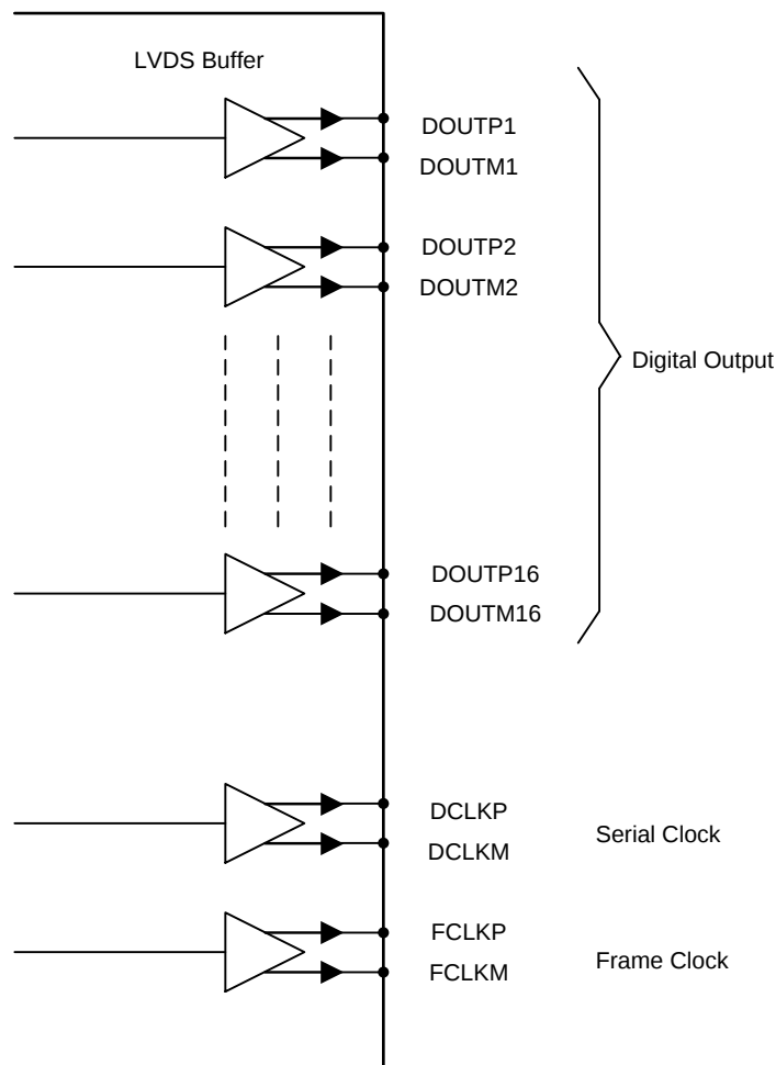
Figure 75. LVDS Output
