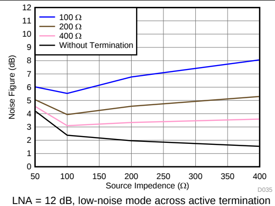
Figure 35. Noise Figure vs Source Impedance
