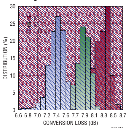
10GHz Conversion Loss Histogram
