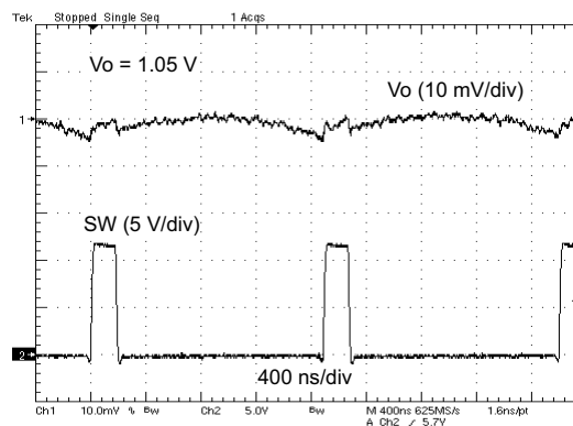
Figure 12. VOLTAGE RIPPLE AT OUTPUT ( I_O = 2\text{ A} )
