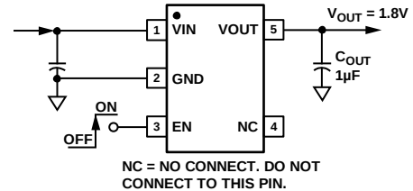
Figure 1. ADP150UJZ-RedyKit
