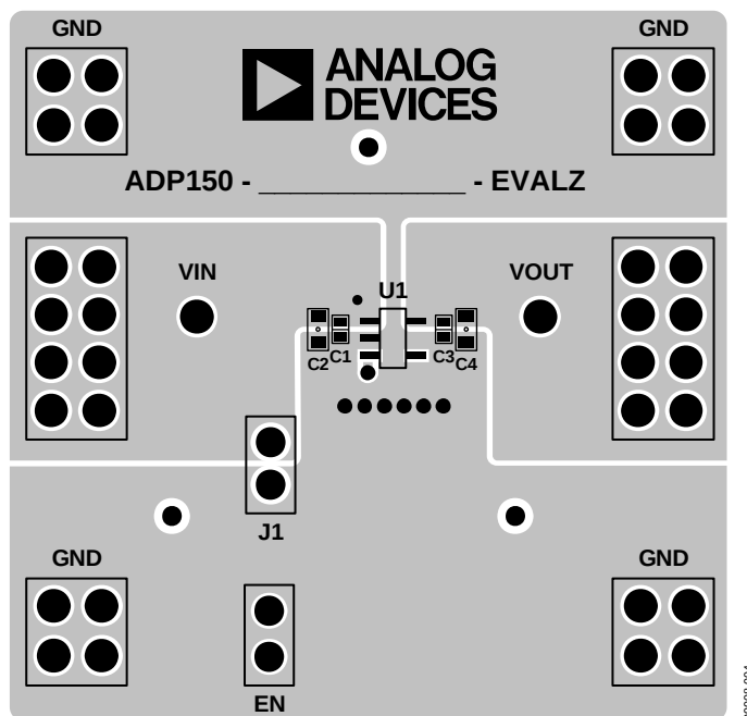
Figure 4. ADP150UJZ-RedyKit Evaluation Board Layout
