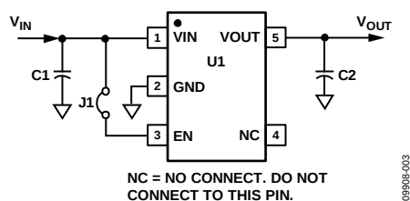
Figure 3. ADP150UJZ-RedyKit Evaluation Board Schematic
