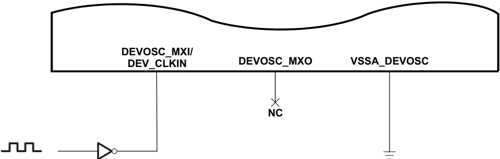
Figure 7-10. 1.8-V LVC MOS-Compatible Clock Input (DEV_OSC)
