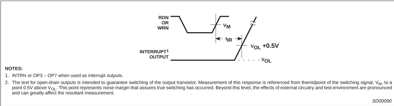
Figure 6. Interrupt Timing
