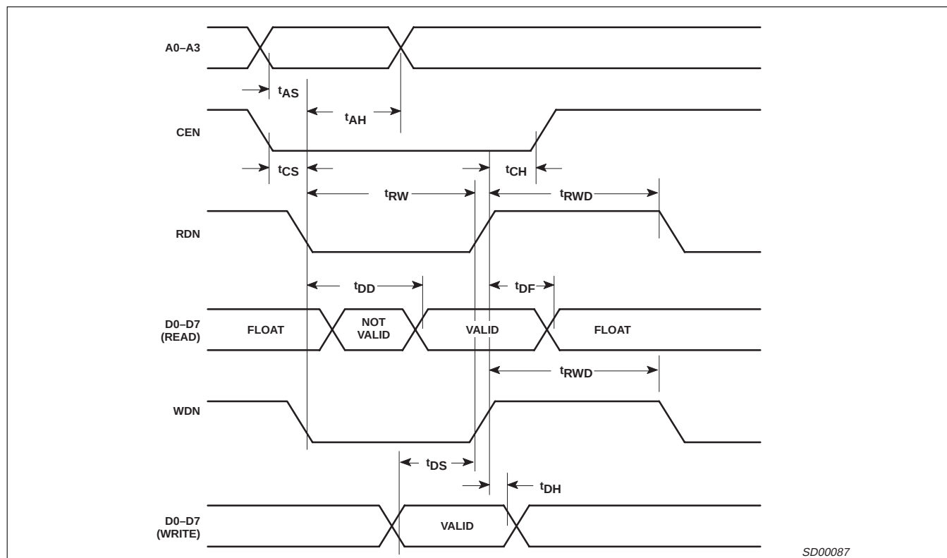
Figure 4. Bus Timing
