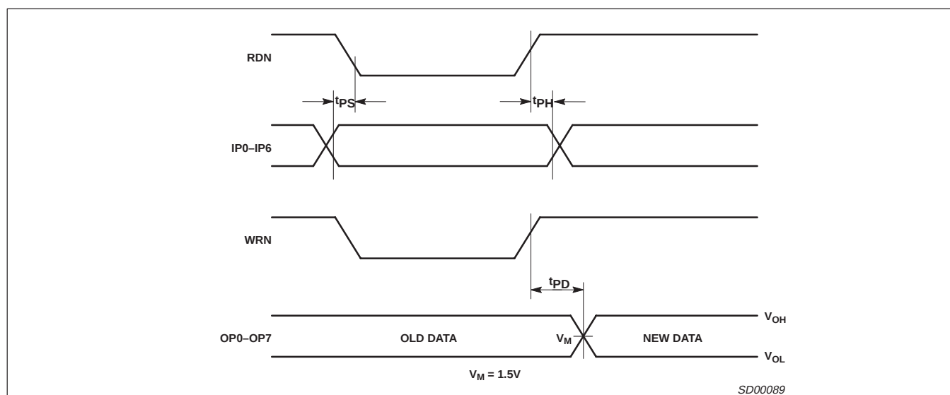
Figure 5. Port Timing
