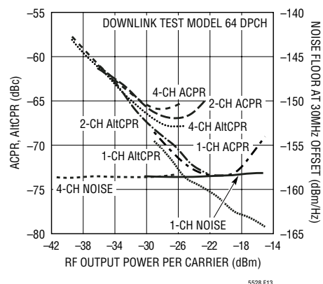
Figure 13: W-CDMA ACPR, AltCPR and Noise vs RF Output Power at 2140MHz for 1, 2 and 4 Channels
