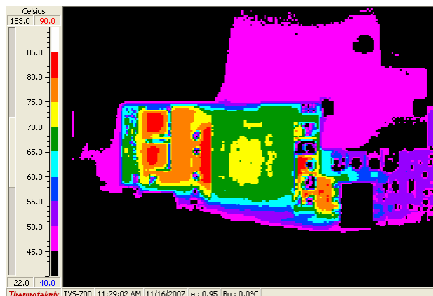
Figure 8. Temp Data (36Vin, 12Aout, 25°C, 200LFM airflow – front)
