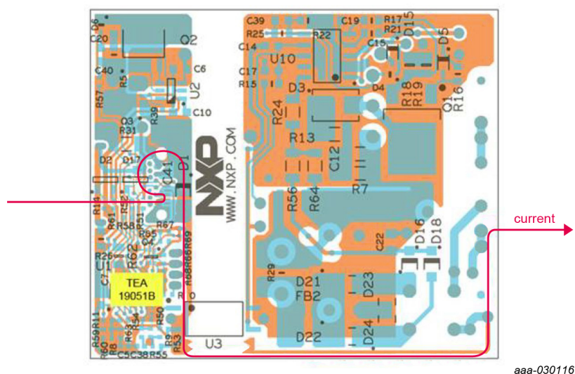
Figure 22. Low ohmic, short ESD connection between USB port and mains
