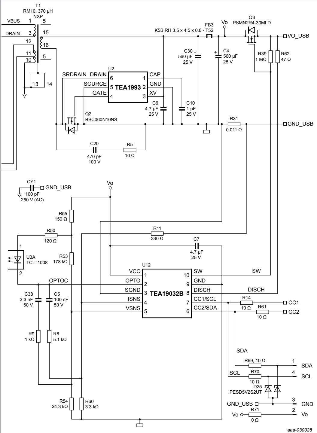
Figure 10. Secondary side of the 65 W demo board
