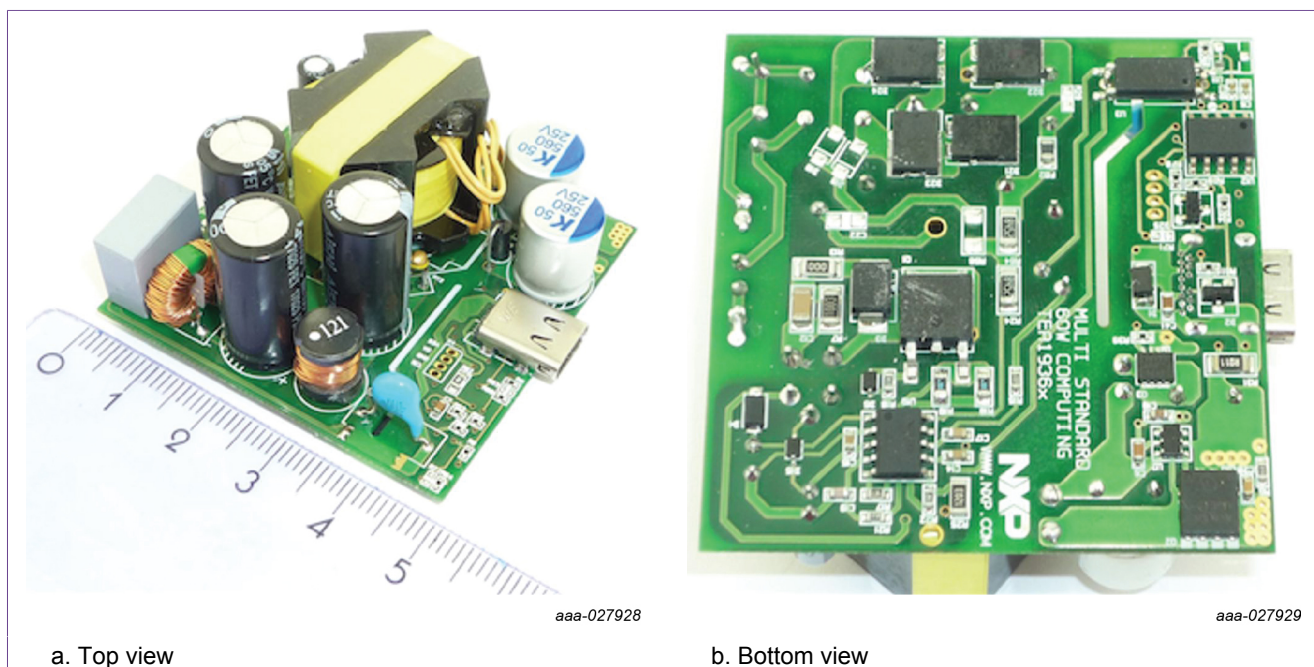
Figure 24. Demo PCB of a multistandard 60 W computing charging demo board (50 mm × 50 mm × 25 mm) with TEA19032B, TEA19361, and TEA1993
