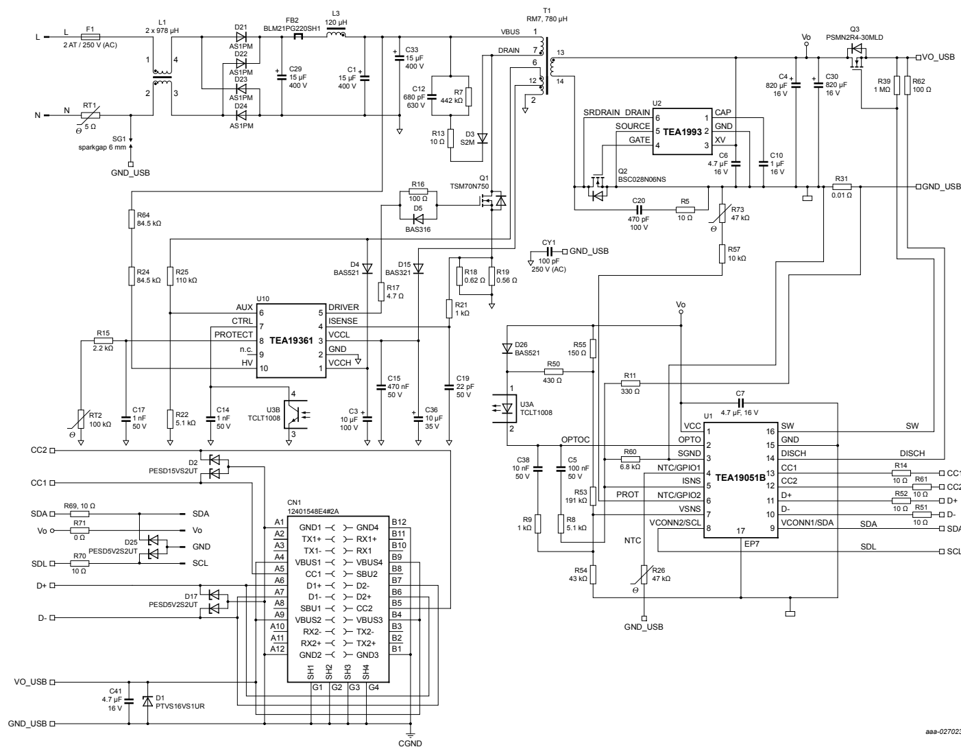
Figure 23. TEA1936DB1475 27 W QC4+ reference design
