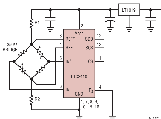
Figure 47. Simple Bridge Connection
