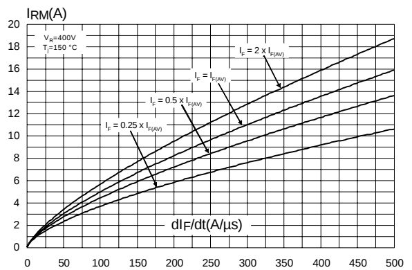
Figure 4: Peak reverse recovery current versus di/dt (typical values)
