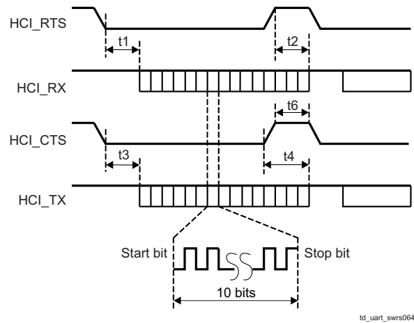
Figure 5-2. UART Timing
