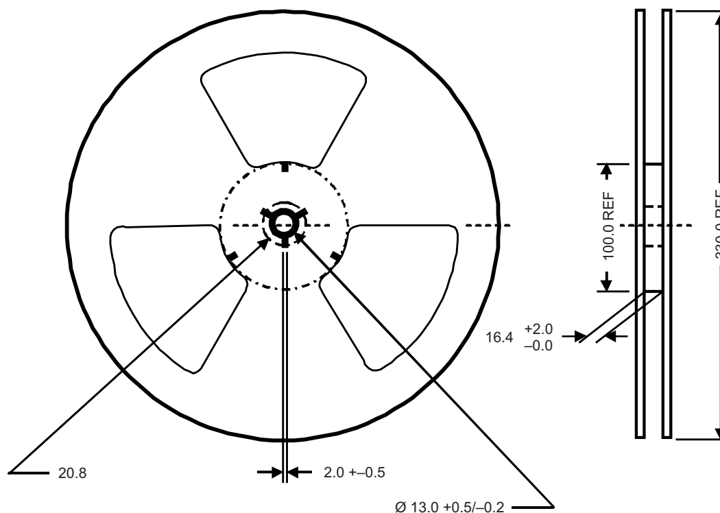
Figure 9-5. Reel Dimensions (mm)
