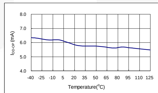
Figure 10. Operating Current
