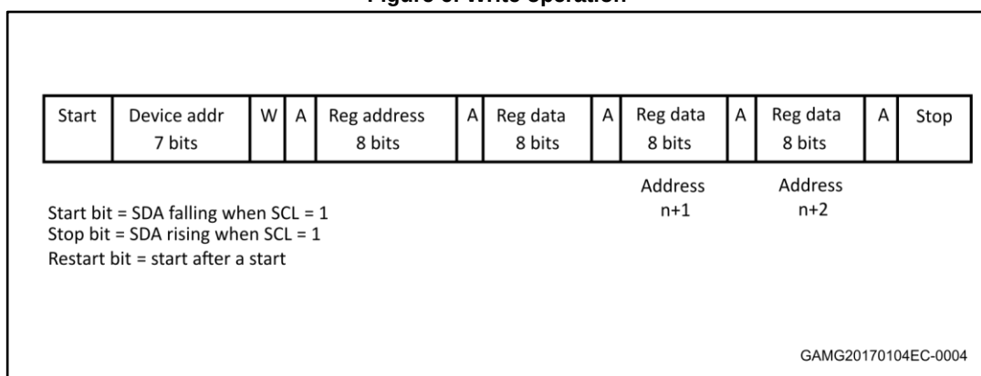
Figure 6: Write operation
