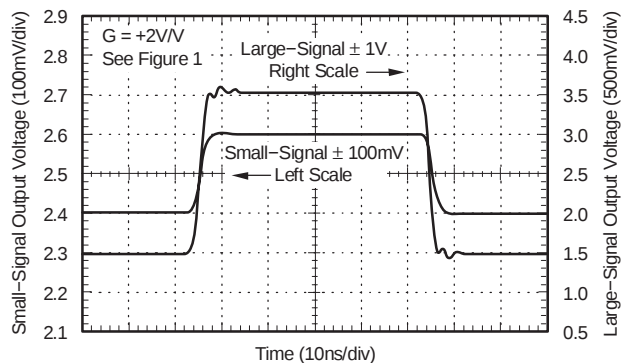
NONINVERTING PULSE RESPONSE
