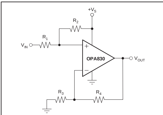
Figure 4. DC Level-Shifting
