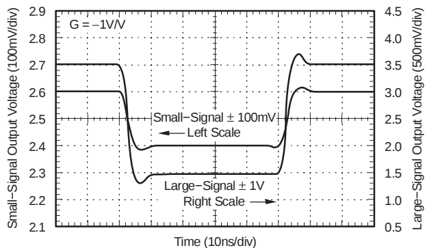
INVERTING PULSE RESPONSE
