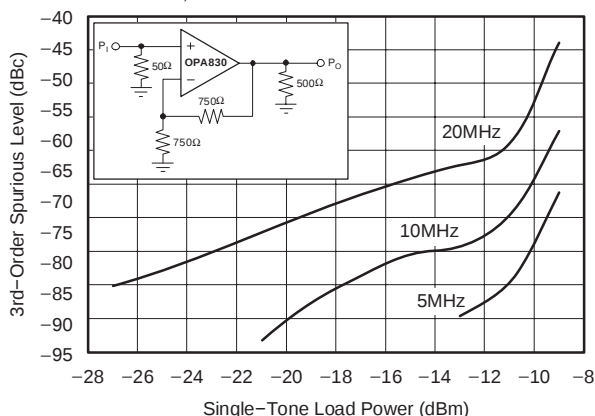
TWO-TONE, 3RD-ORDER INTERMODULATION SPURIOUS
