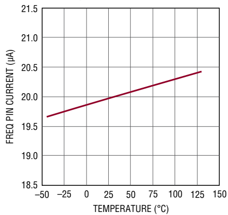
FREQ Pin Source Current vs Temperature
