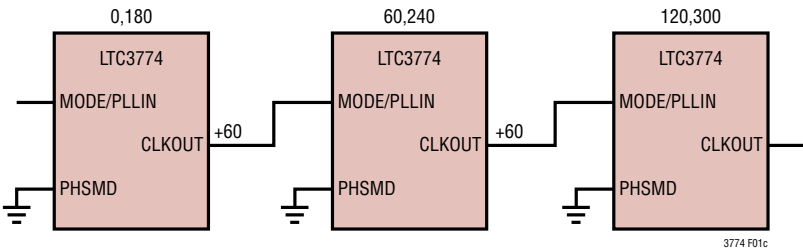
Figure 1c. 6-Phase Operation
