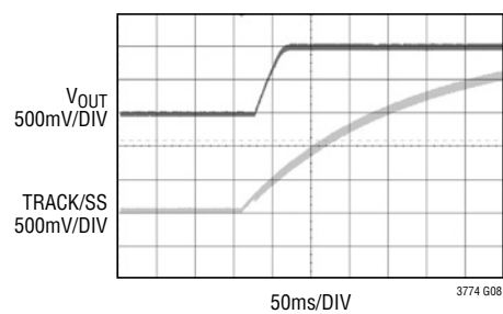
Prebiased Output at 0.5V
