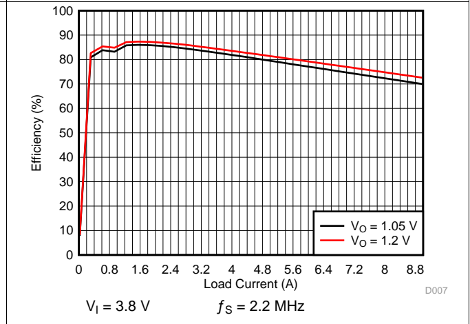
Figure 4-7. SMPS Efficiency for 9-A Multi-Phase PWM Mode
