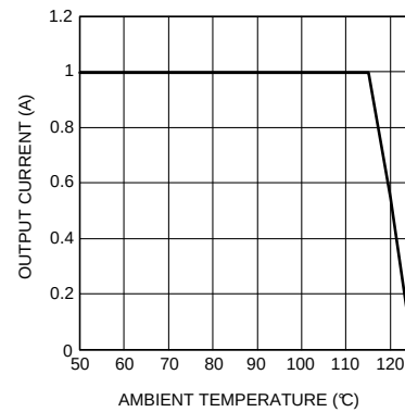
Figure 40. Thermal Derating Curve
