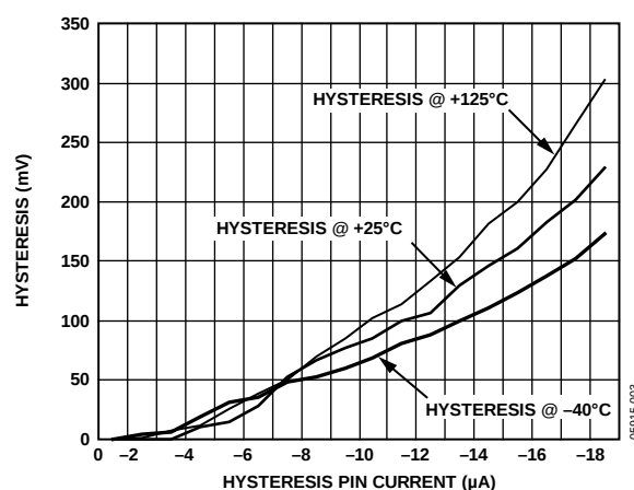
Figure 9. Hysteresis vs. Hysteresis Pin Current
