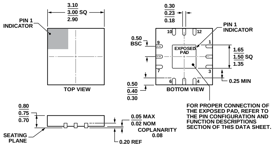
Figure 25. 12-Lead Lead Frame Chip Scale Package [LFCSP] 3 mm × 3 mm Body and 0.75 mm Package Height (CP-12-5)
