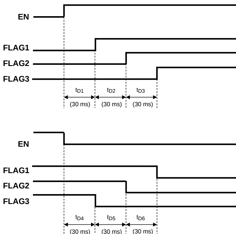
Figure 1. Timing Sequence
