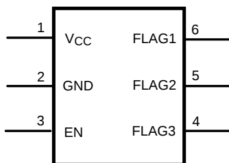
Figure 3. Pin-Out
