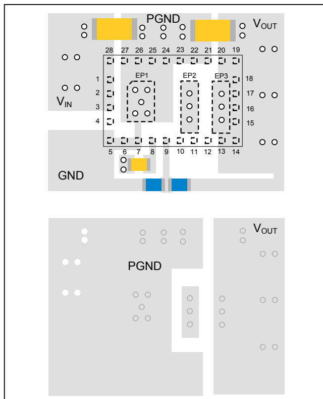
Figure 2. Layout Recommendation
