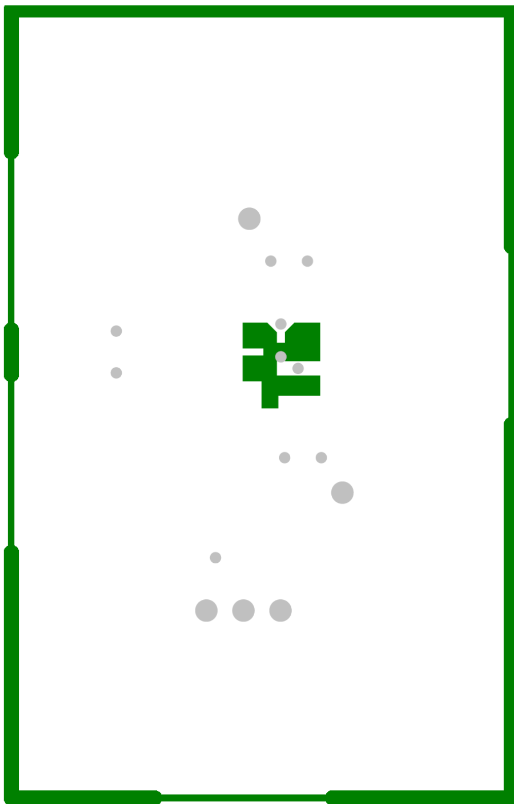
Figure 3. OPA837DCKEVM Layer 2
