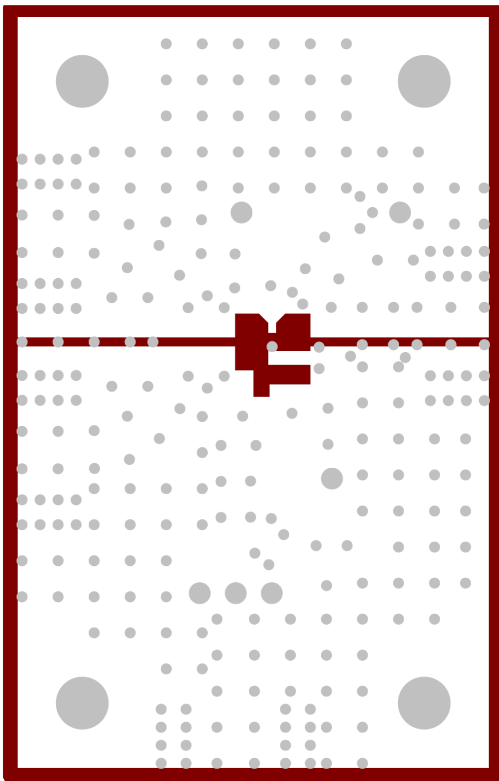
Figure 4. OPA837DCKEVM Layer 3
