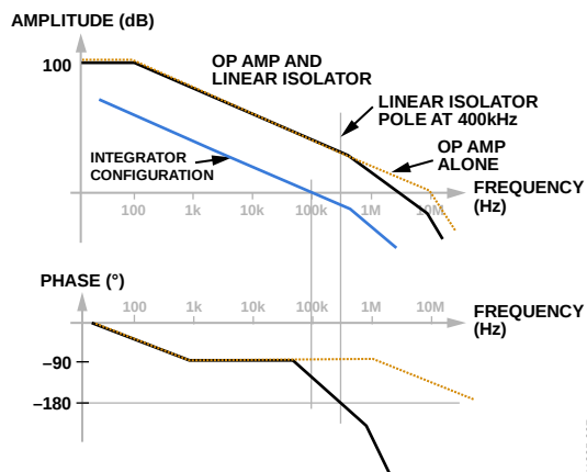
Figure 31. Bode Plot 2
