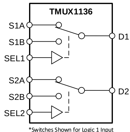
Block Diagram
