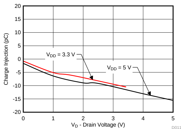
Figure 28. Charge Injection vs Drain Voltage
