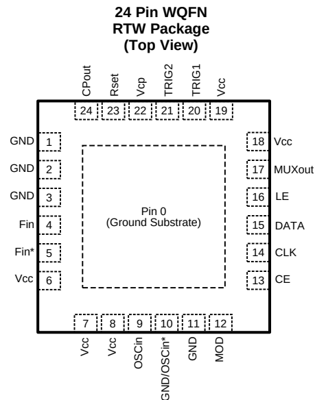
Pin Functions
