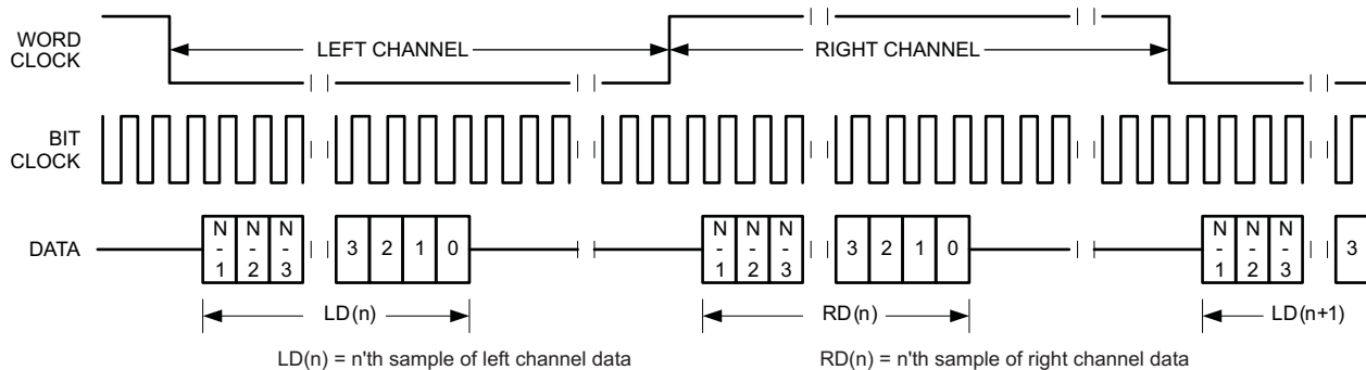
Figure 2-15. Timing Diagram for I²S Mode
