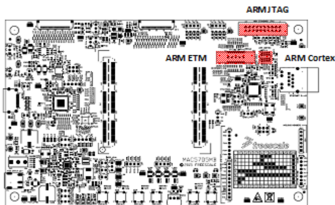
Figure 4. Debug connectors
