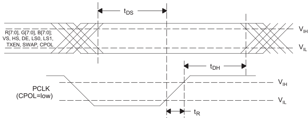
Figure 8. Setup/Hold Time
