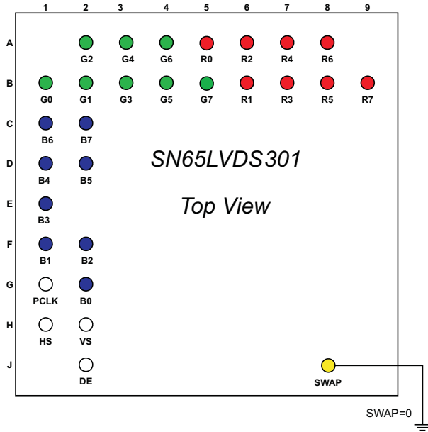
Figure 1. SWAP PIN = 0
