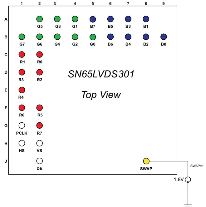
Figure 2. SWAP PIN = 1
