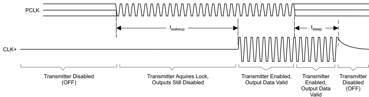
Figure 16. Standby Detection
