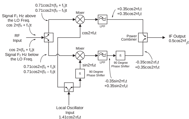
Figure 5. Image Reject Mixer
