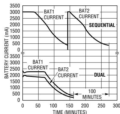
Dual vs Sequential Charging
