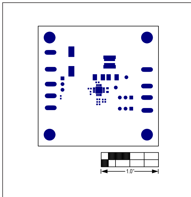
Figure 17. MAX17505 3.3V Output EV Kit Component Placement Guide—Top Solder Mask
