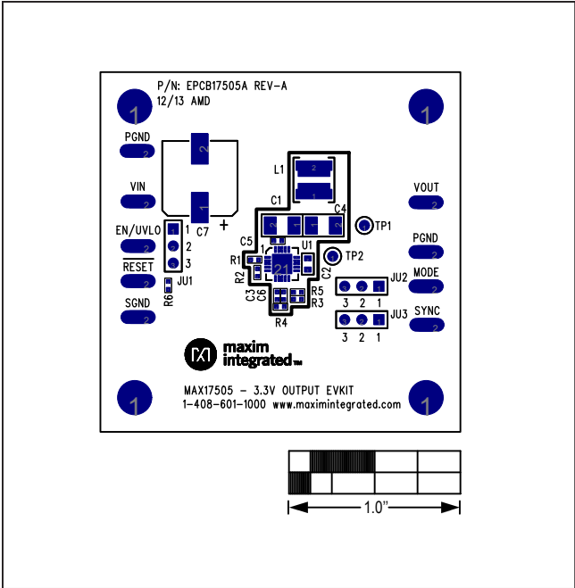
Figure 12. MAX17505 3.3V Output EV Kit Component Placement Guide—Component Side
