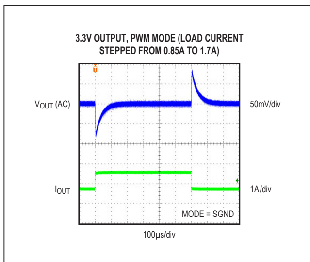
Figure 10. MAX17505 3.3V Output, 0.85A to 1.7A Load Transient
