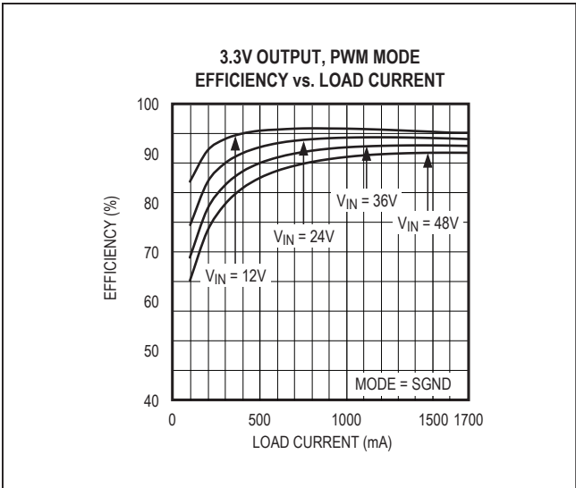
Figure 2. MAX17505 3.3V Output Efficiency (PWM Mode)
