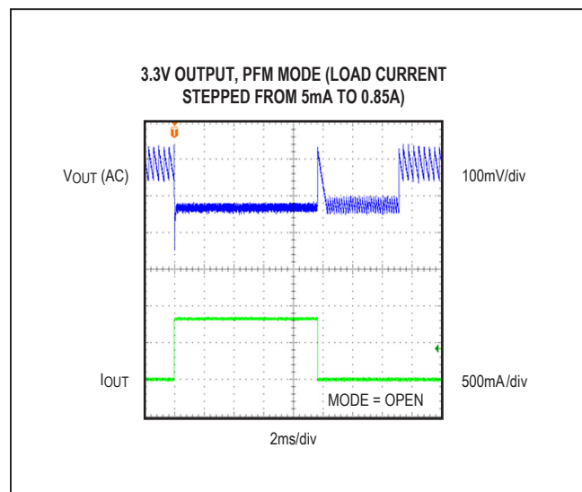
Figure 8. MAX17505 3.3V Output, 5mA to 0.85A Load Transient (PFM Mode)
