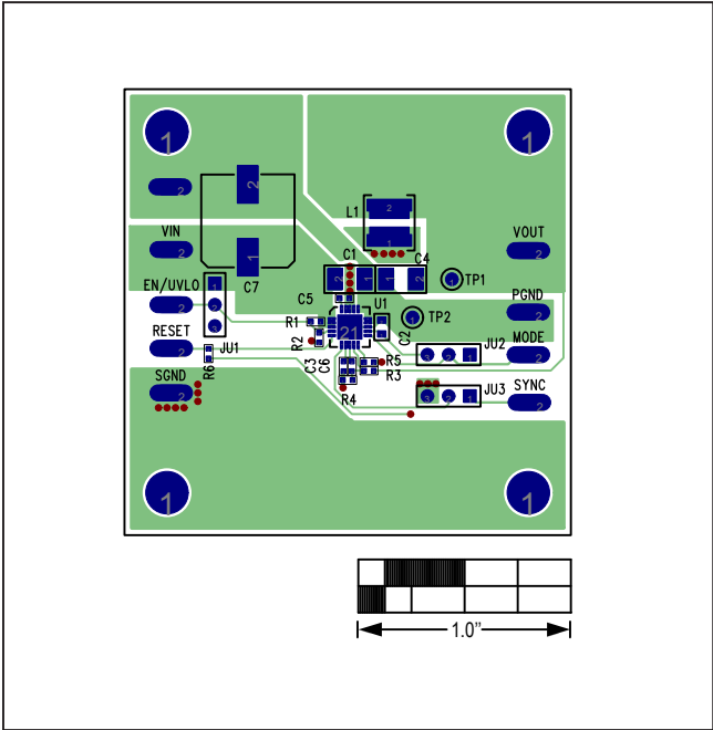
Figure 13. MAX17505 3.3V Output EV Kit Component Side PCB layout
