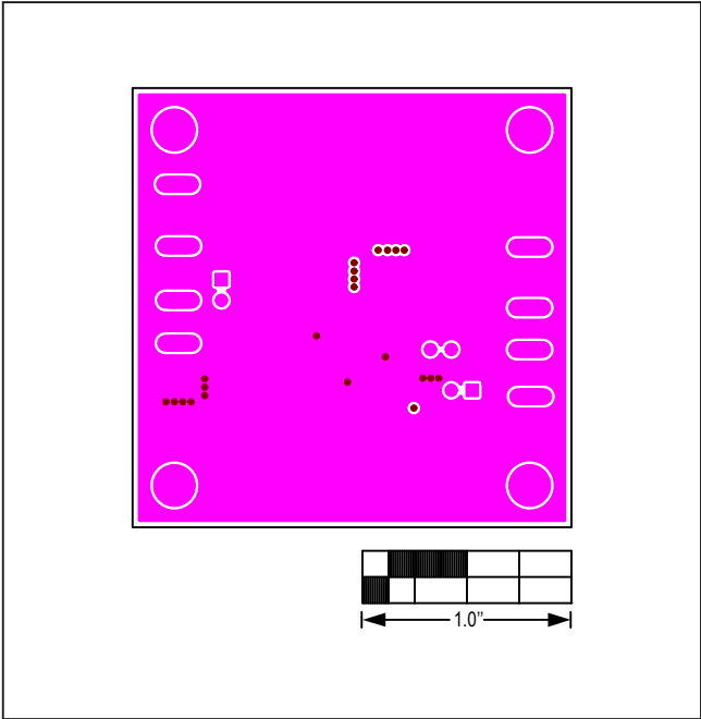
Figure 15. MAX17505 3.3V Output EV Kit PCB Layout—Inner Layer 2
