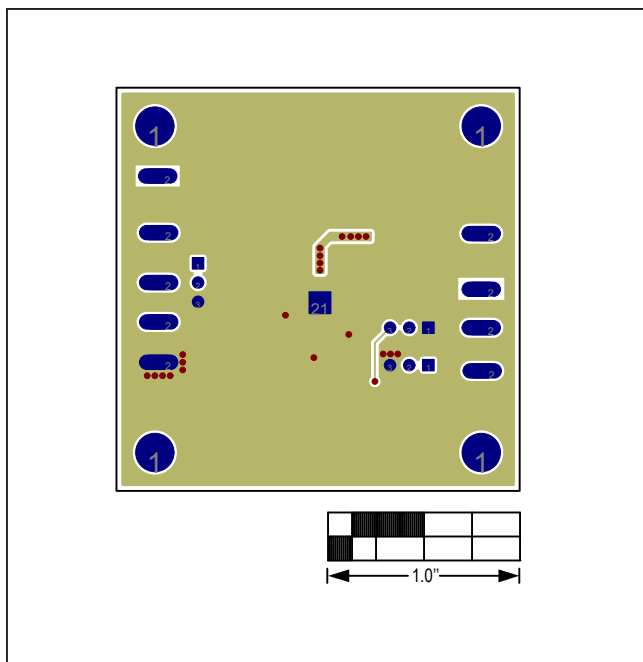
Figure 16. MAX17505 3.3V Output EV Kit PCB Layout— Solder Side
