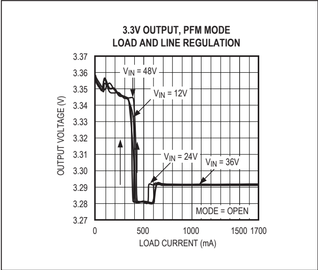
Figure 3. MAX17505 3.3V Output Load and Line Regulation (PFM Mode)
