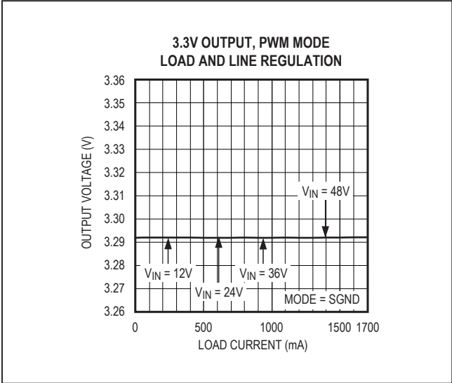
Figure 1. MAX17505 3.3V Output Load and Line Regulation (PWM Mode)
