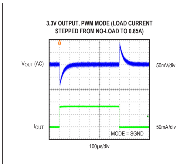
Figure 7. MAX17505 3.3V Output, No Load to 0.85A Load Transient (PWM Mode)
