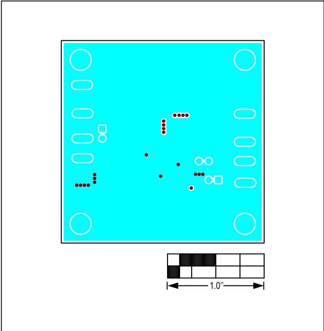
Figure 14. MAX17505 3.3V Output EV Kit PCB Layout—Inner Layer 1
