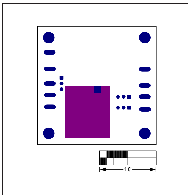
Figure 18. MAX17505 3.3V Output EV Kit Component Placement Guide—Bottom Solder Mask
