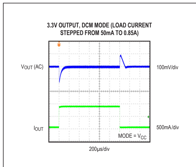
Figure 9. MAX17505 3.3V Output, 50mA to 0.85A Load Transient (DCM Mode)
