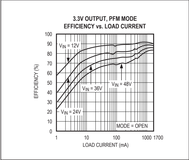
Figure 4. MAX17505 3.3V Output Efficiency (PFM Mode)
