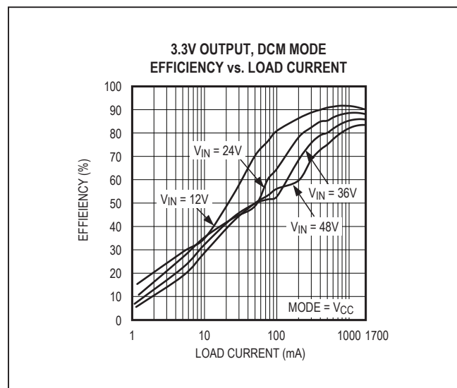
Figure 5. MAX17505 3.3V Output Efficiency (DCM Mode)
