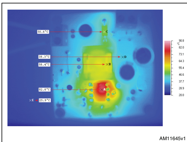
Figure 22. Thermal map at V_{IN} = 265\text{ V}_{AC} , I_{out} = 350\text{ mA} , T_{AMB} = 25\text{ }^{\circ}\text{C} : IC self supplied (J1 not selected)
