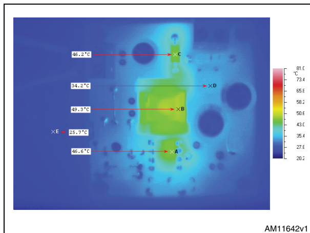
Figure 19. Thermal map at V_{IN} = 230\text{ V}_{AC} , I_{out} = 350\text{ mA} , T_{AMB} = 25\text{ }^{\circ}\text{C} : IC supplied from the output (J1 selected)
