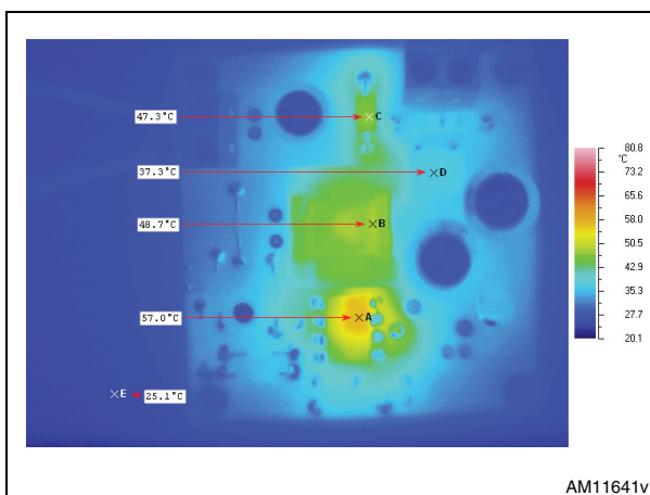
Figure 18. Thermal map at V IN = 115 V AC , I out = 350 mA, T AMB = 25 °C: IC self supplied (J1 not selected)
