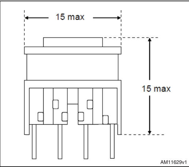
Figure 6. Transformer size side view 2
