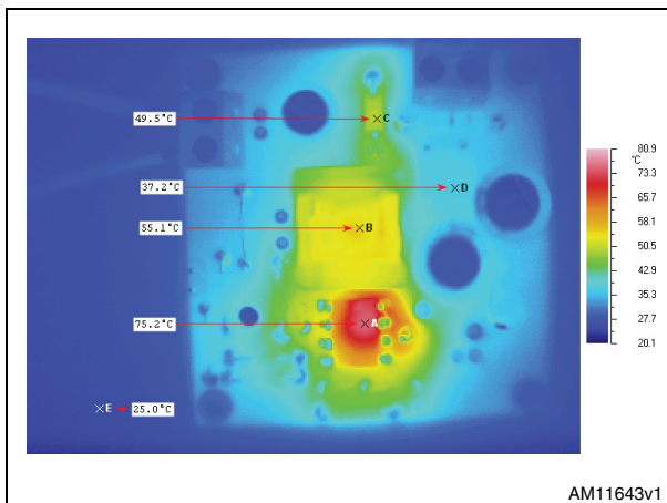
Figure 22. Thermal map at V_{IN} = 265\text{ V}_{AC} , I_{out} = 350\text{ mA} , T_{AMB} = 25\text{ }^{\circ}\text{C} : IC self supplied (J1 not selected)
