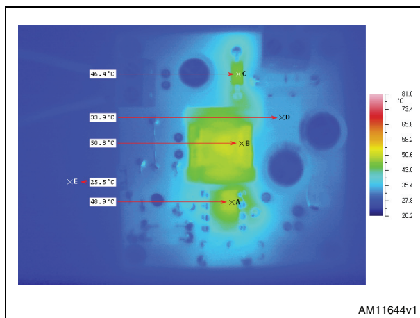
Figure 21. Thermal map at V_{IN} = 265\text{ V}_{AC} , I_{out} = 350\text{ mA} , T_{AMB} = 25\text{ }^{\circ}\text{C} : IC supplied from the output (J1 selected)
