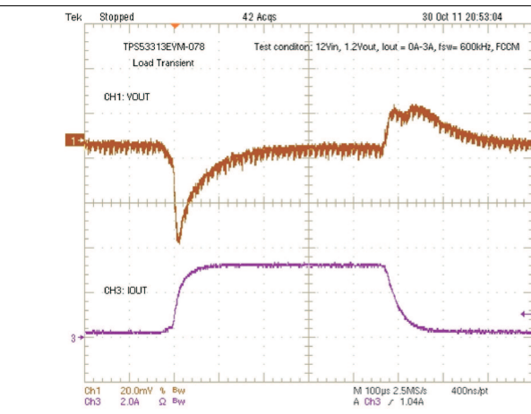
Figure 20. Output Load, 0-A to 3-A Transient Under FCCM Mode
