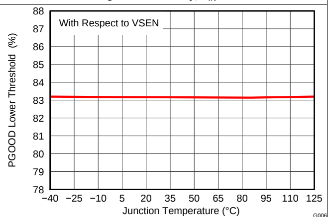
Figure 6. PGOOD Lower Threshold vs Junction Temperature
