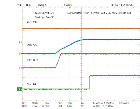
Figure 22. Start-Up Waveform
