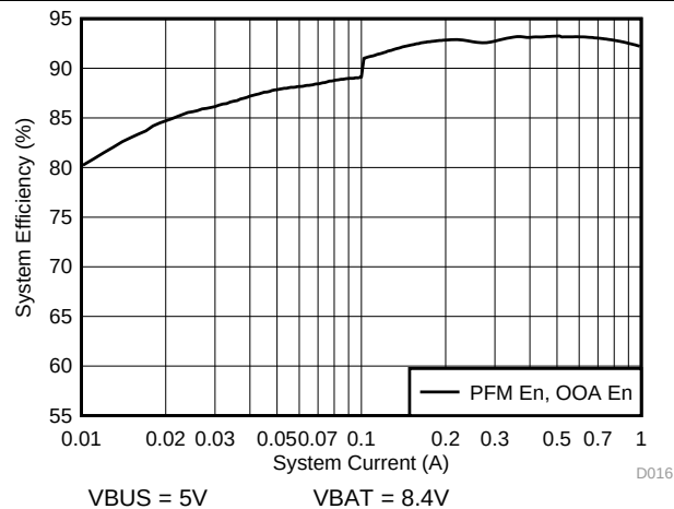
Figure 3. System Efficiency vs. System Current
