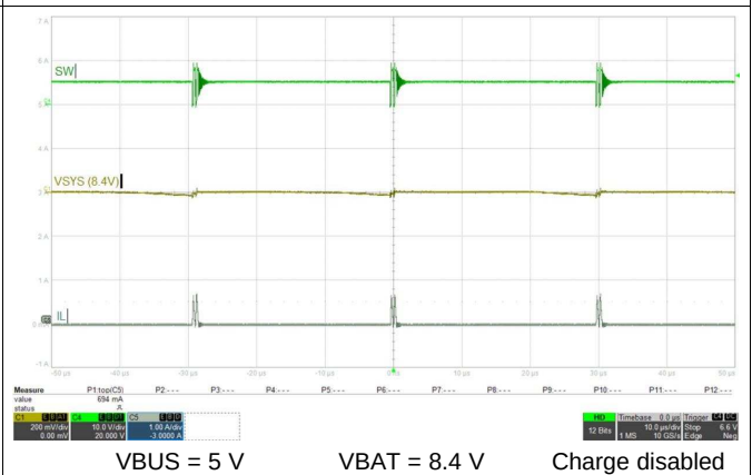
Figure 30. Boost Mode PFM Switching
