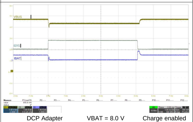
Figure 32. VINDPM Transient Response
