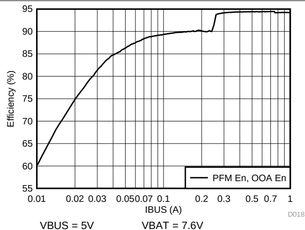
Figure 5. OTG Efficiency vs. VBUS Output Current
