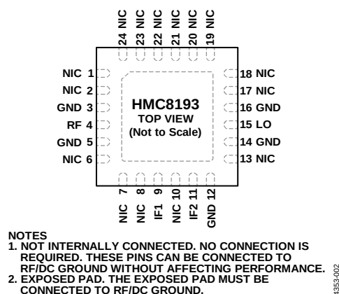
Figure 2. Pin Configuration
