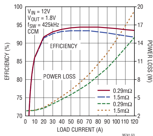
Efficiency and Power Loss vs Output Current (4-Phase with Master Controller LTC3884-1)
