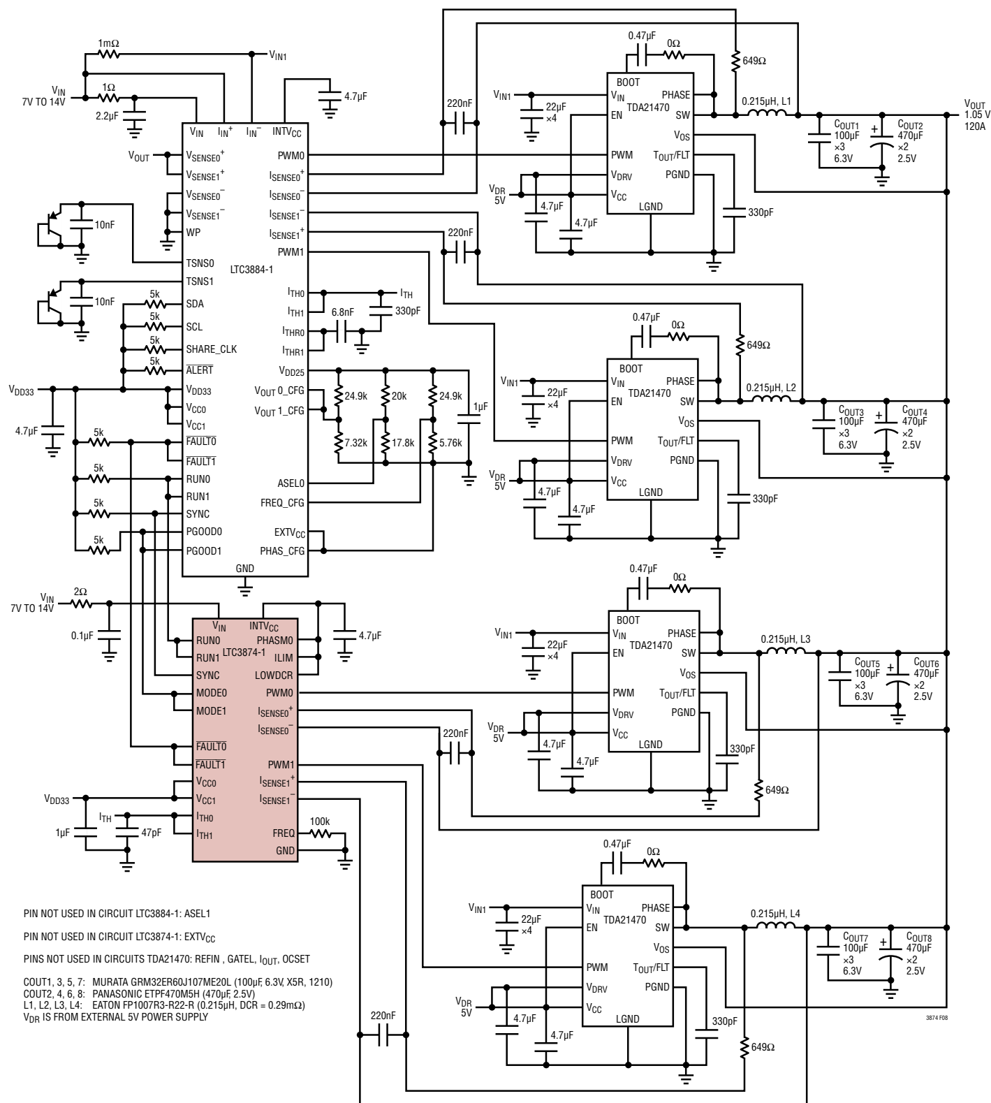
Figure 8. High Efficiency 500kHz 4-Phase 1.05V Step-Down Converter
