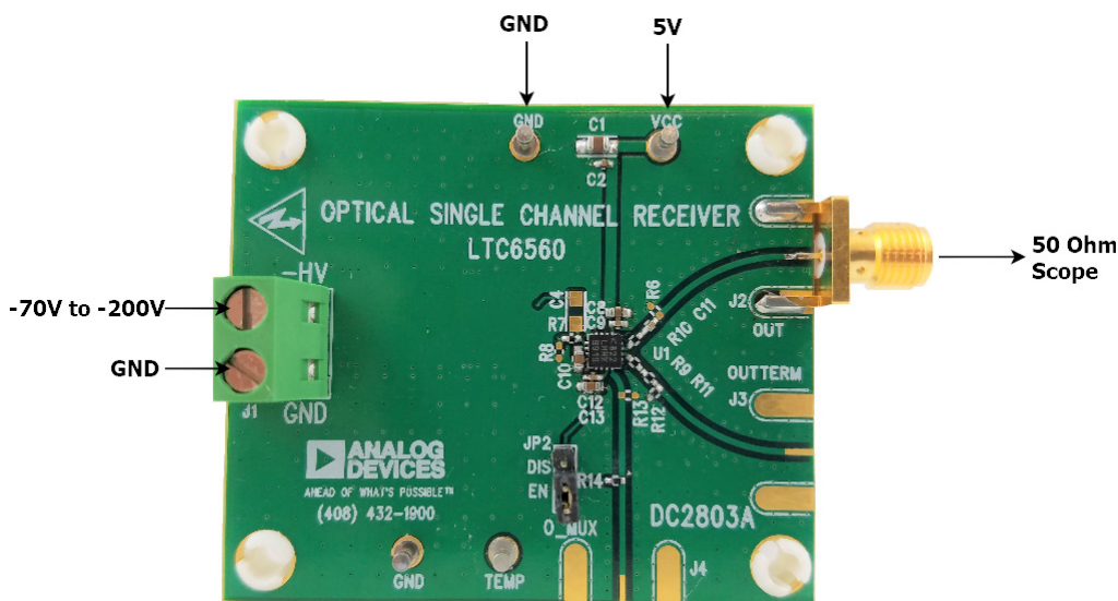
Figure 1. Connection Diagram
