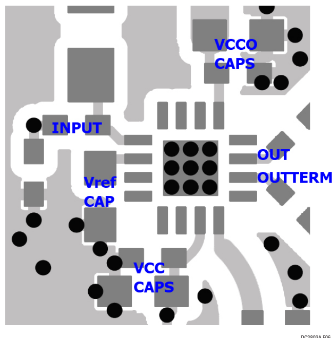
Figure 6. Recommended Layout
