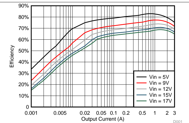
Figure 10. Efficiency vs Output Current, V OUT = 0.9 V 0.9 V Efficiency L = 0.56 μH (Wurth:7443835600 56)
