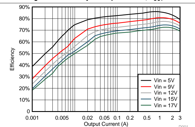
Figure 12. Efficiency vs Output Current, V OUT = 1.2 V 1.2 V Efficiency L = 0.68 μH (Wurth:7443835600 68)
