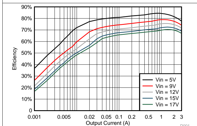
Figure 11. Efficiency vs Output Current, V OUT = 1.05 V 1.05 V Efficiency L = 0.56 μH (Wurth:7443835600 56)
