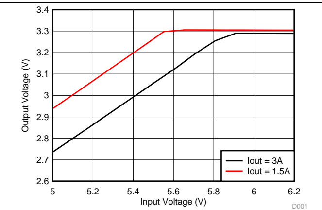
Figure 8. Dropout for 3.3 V Output Voltage
