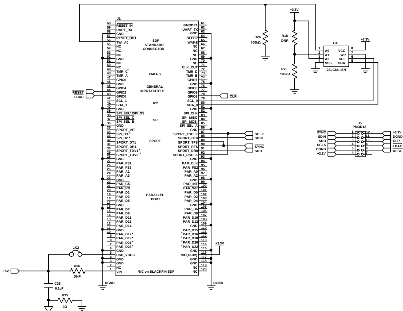
Figure 12. Schematic of the EVAL-SDP-CB1Z SDP-B Board Connector
