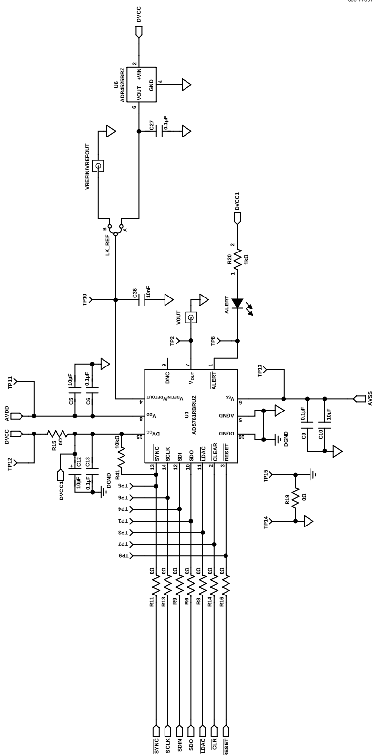
Figure 9. Schematic of the AD5761RSDZ Circuitry
