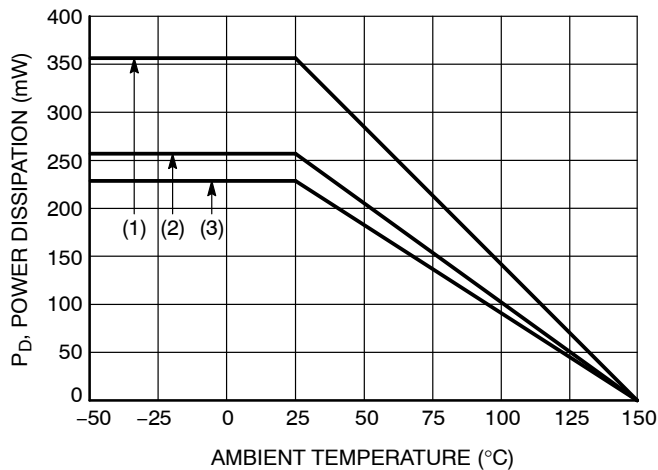
Figure 77. Derating Curve
