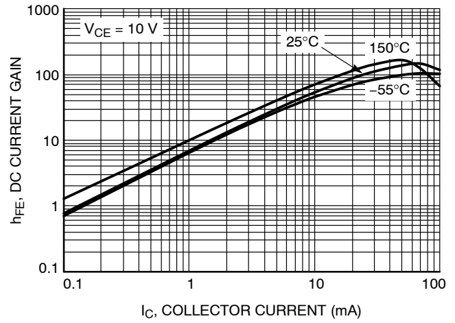
Figure 89. DC Current Gain
