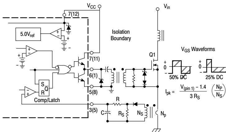
Figure 30. Isolated MOSFET Drive
