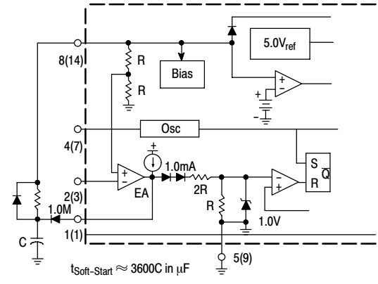
Figure 24. Soft-Start Circuit
