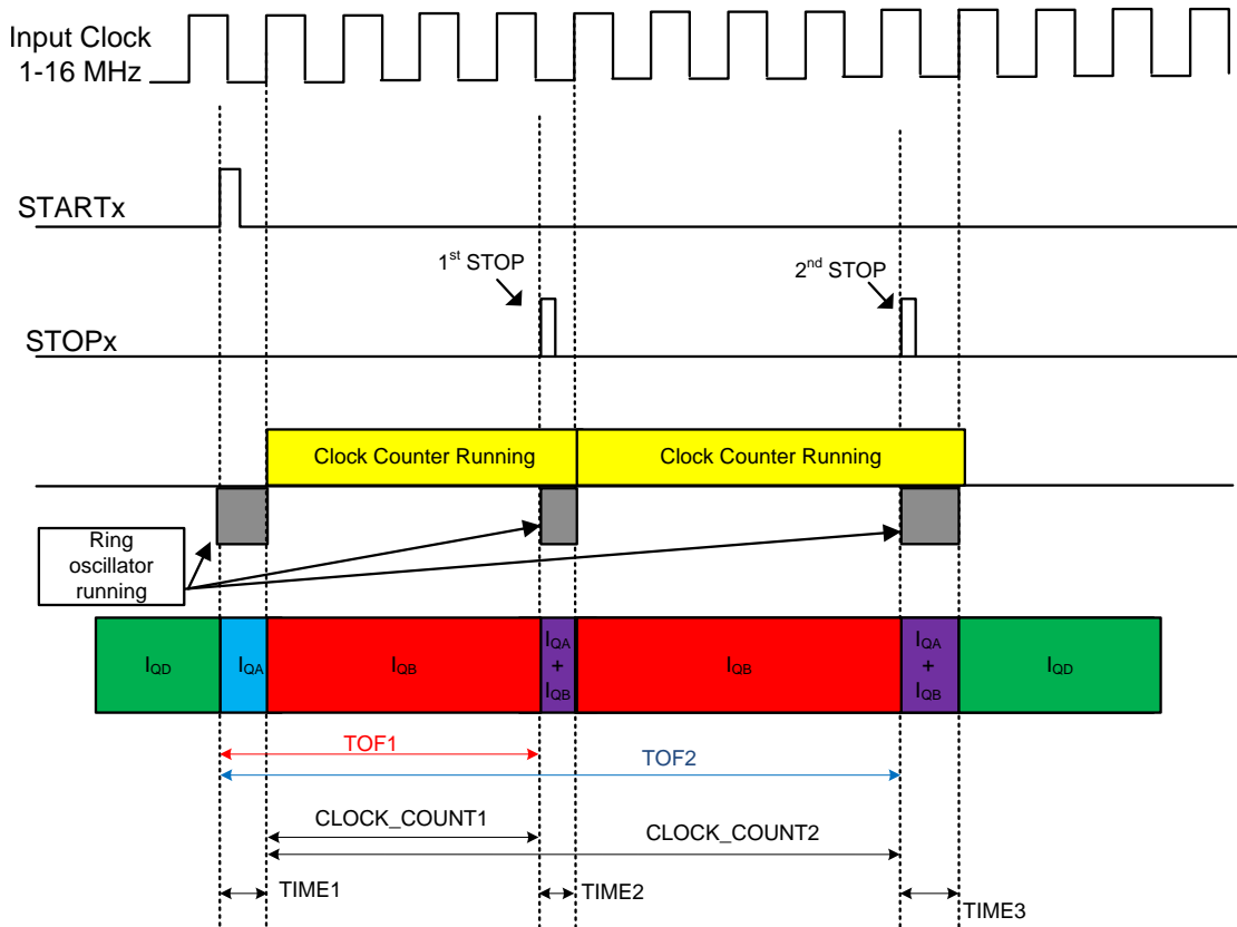
Figure 23. Measurement Mode 2
