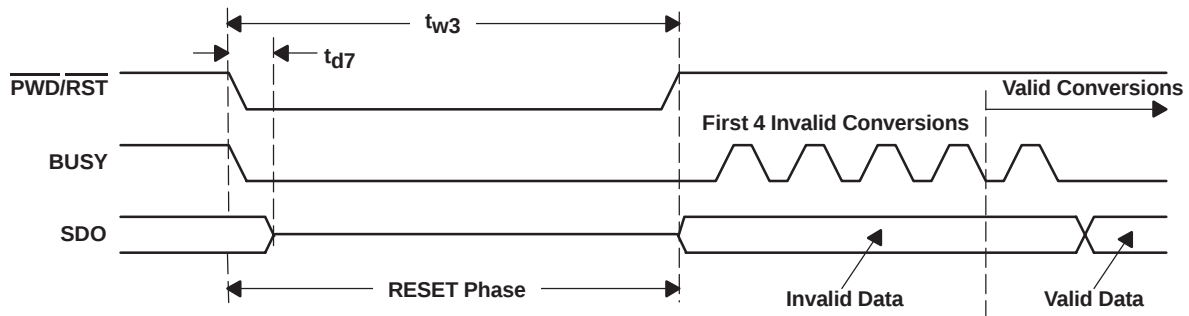
Figure 4. Device Reset
