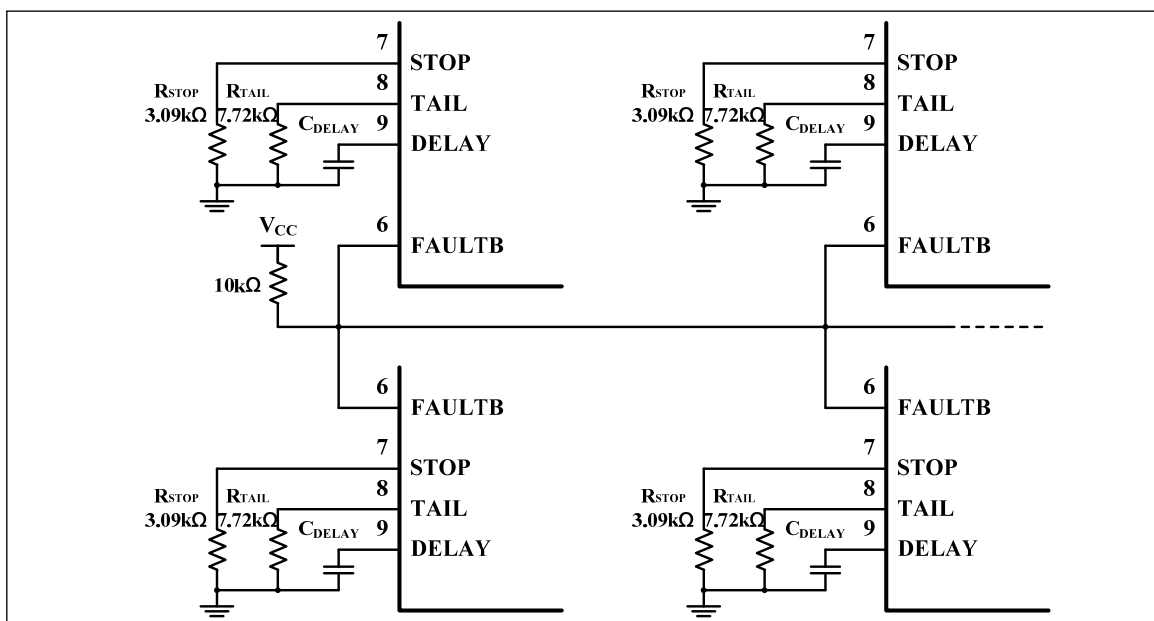
Figure 3 Several Devices Connect FAULTB Pin In Parallel
