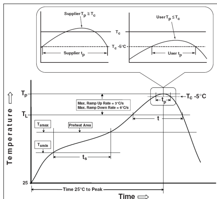
Figure 31 Classification Profile
