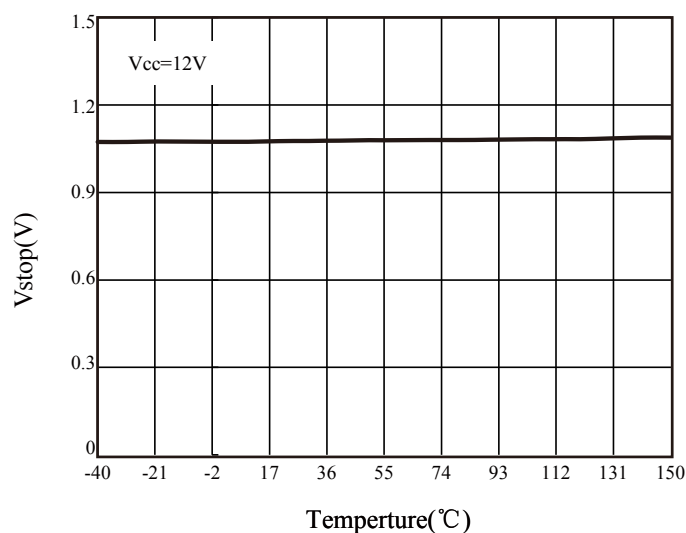
Figure 13 V_STOP vs. Temperature
