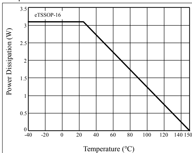
Figure 29 Dissipation Curve
