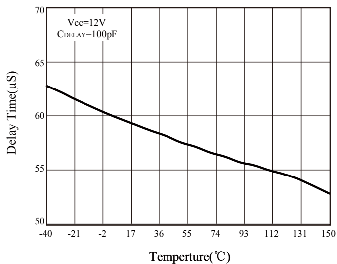
Figure 11 Delay Time vs. Temperature
