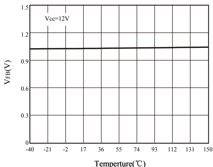
Figure 15 V_FB vs. Temperature
