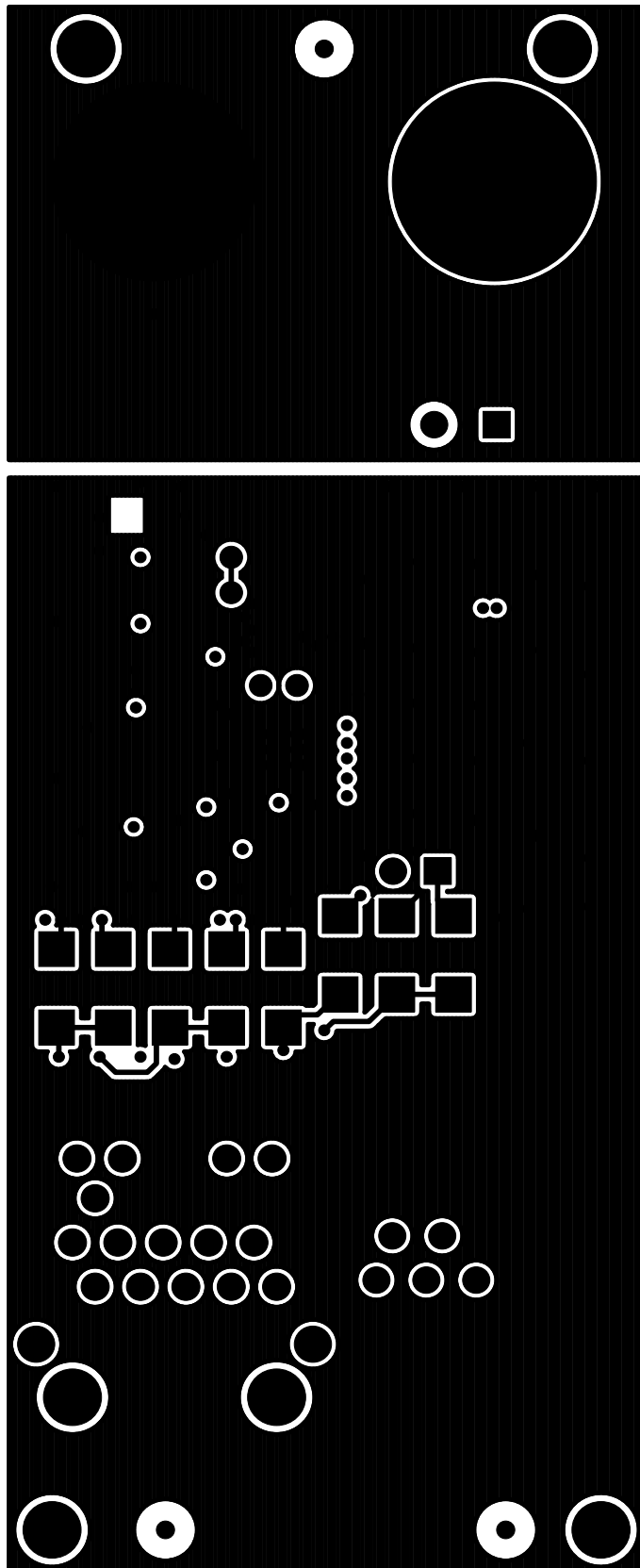
Figure 6. Bottom Layer
