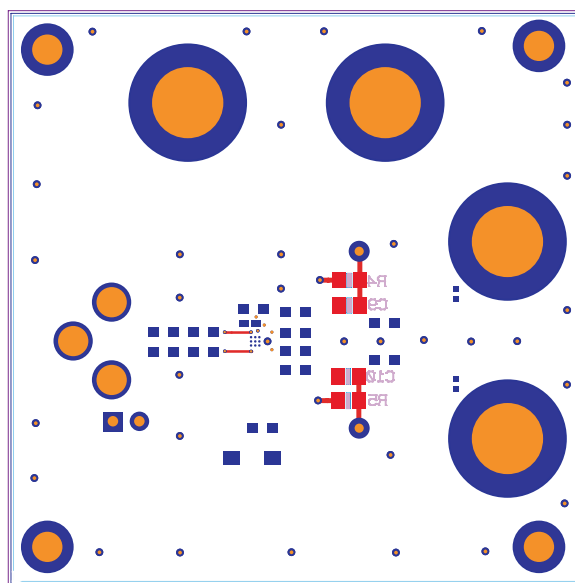
Figure 2. Bottom Layer
