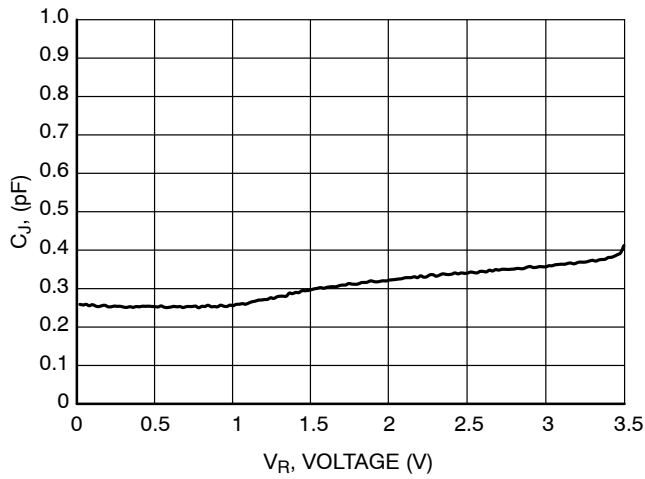
Figure 9. Junction Capacitance; V_R = 3.5 V – 0 V, f = 1 MHz, I/O – GND, dV/dt = 214 mV/s
