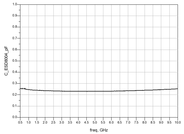
Figure 10. Junction Capacitance; V_R = 0 V, f = 500 MHz – 10 GHz
