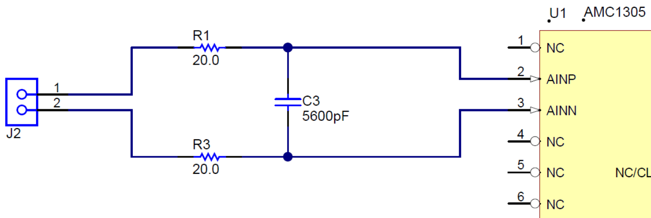
Figure 1. AMC1305EVM Schematic: Analog Input Section
