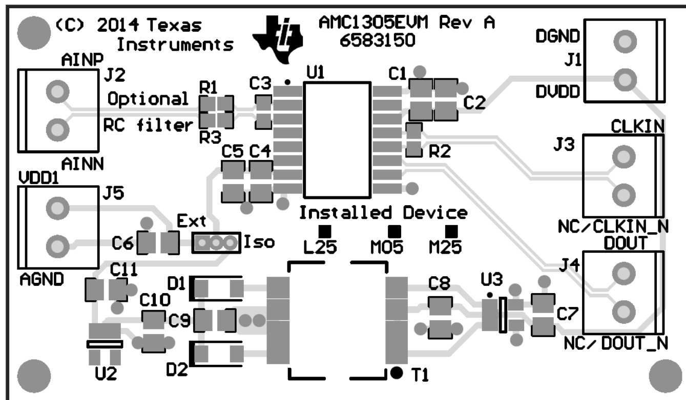
Figure 6. AMC1305EVM Silk Screen Drawing
