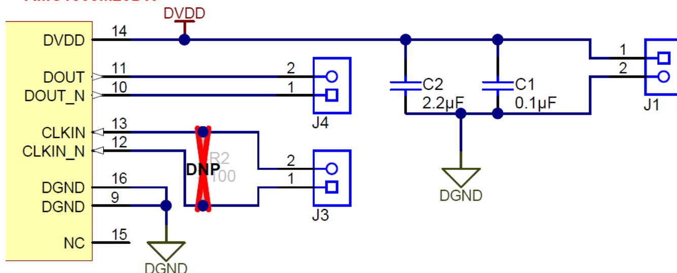
Figure 2. Power, Clock Input, and Digital Data Output
