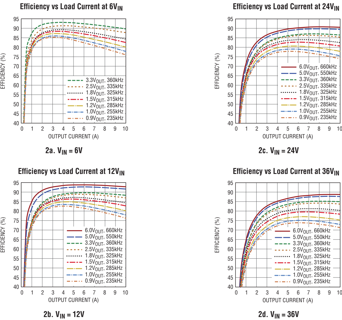
Figure 2. Measured DC1543A Efficiency at Different V_{IN} , V_{OUT} and f_{SW} (CCM Mode Enabled) Please refer to Table 1 in LTM4641 data sheet for the switching frequency at each output voltage.
